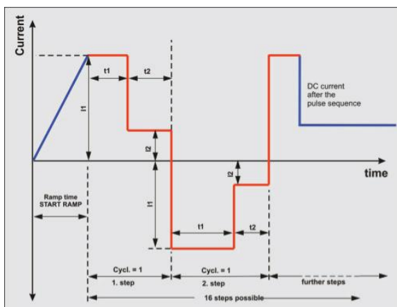
Examples: pulse shapes, schematic display
