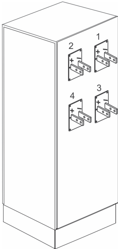
Back panel with pulse output bus bars
